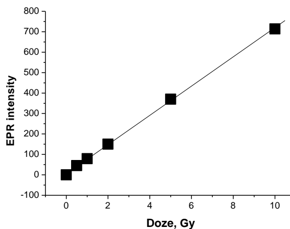
Figure 6. Dependence of EPR signal ( g=2.00 ) intensity of irradiated blood by LINAC.
