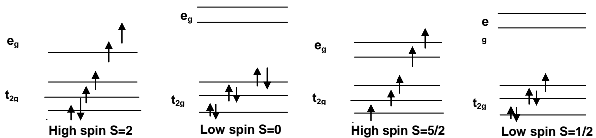
Figure 1. Electronic configuration of \text{Fe}^{2+} (ferrous) [\text{Ar}]3d^6 in low and high spin states in hemoglobin.
