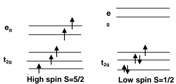
Figure 2. Electronic configuration \text{Fe}^{3+} low and high spin state \text{Fe}^{3+} (ferric) [\text{Ar}]3d^5 .
